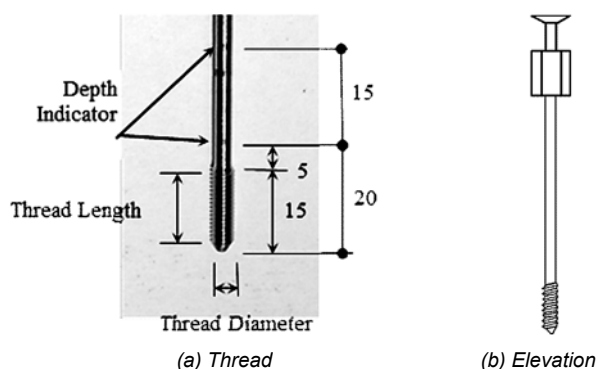
Fig. 1. Standard Probe
